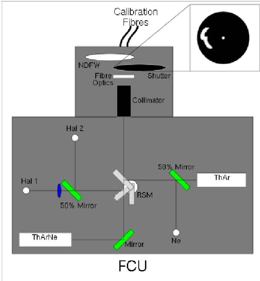
Figure 2.3: Schematic diagram of the FCU.
