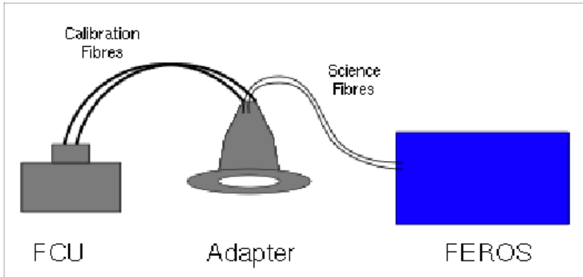
Figure 2.1: Light path of Calibrations.
