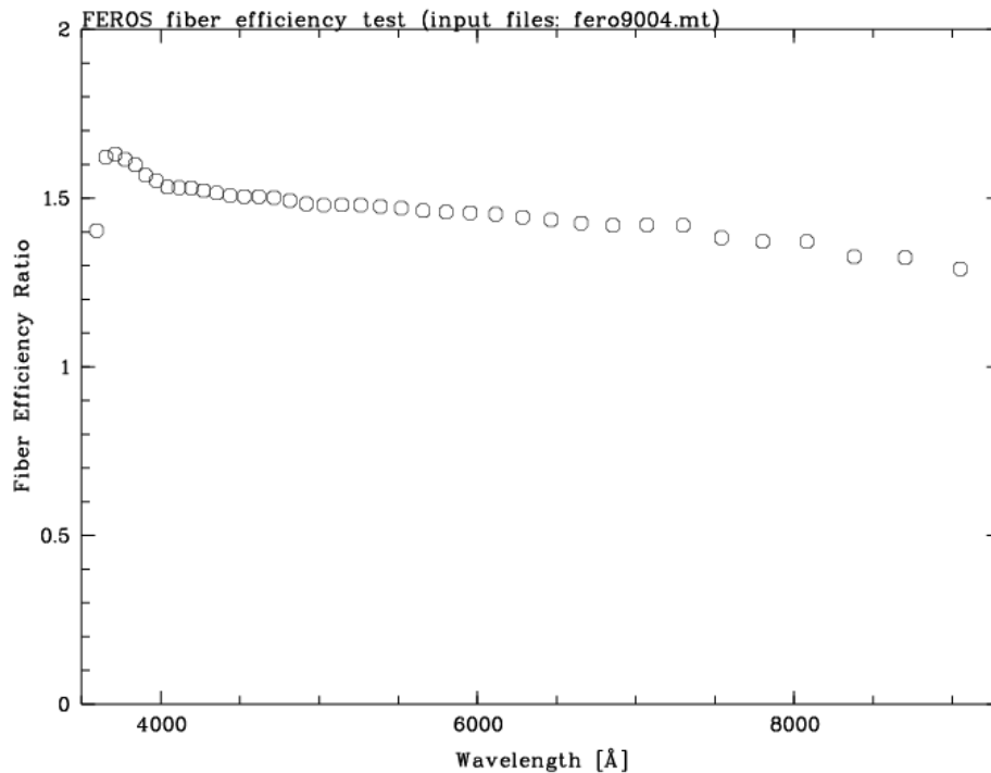
Figure 2.2: The relative fibre efficiency in the sense of OBJECT/SKY fibre. The raw frame is a solar spectrum (image FEROS.2003-11-12T22:42:22.906.fits) acquired during the November Commissioning. Each point represents one of the échelle orders.
