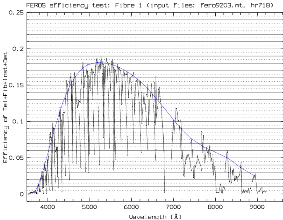
Figure 2.4: The measured efficiency. The raw image is FEROS.2003-11-15T03:46:08.507.fits . The spectrum is a 120 sec exposure of the spectrophotometric standard star HR 718. The blue curve is a polynomial fit to the peak efficiency from each order. Each order is joined by a line.
